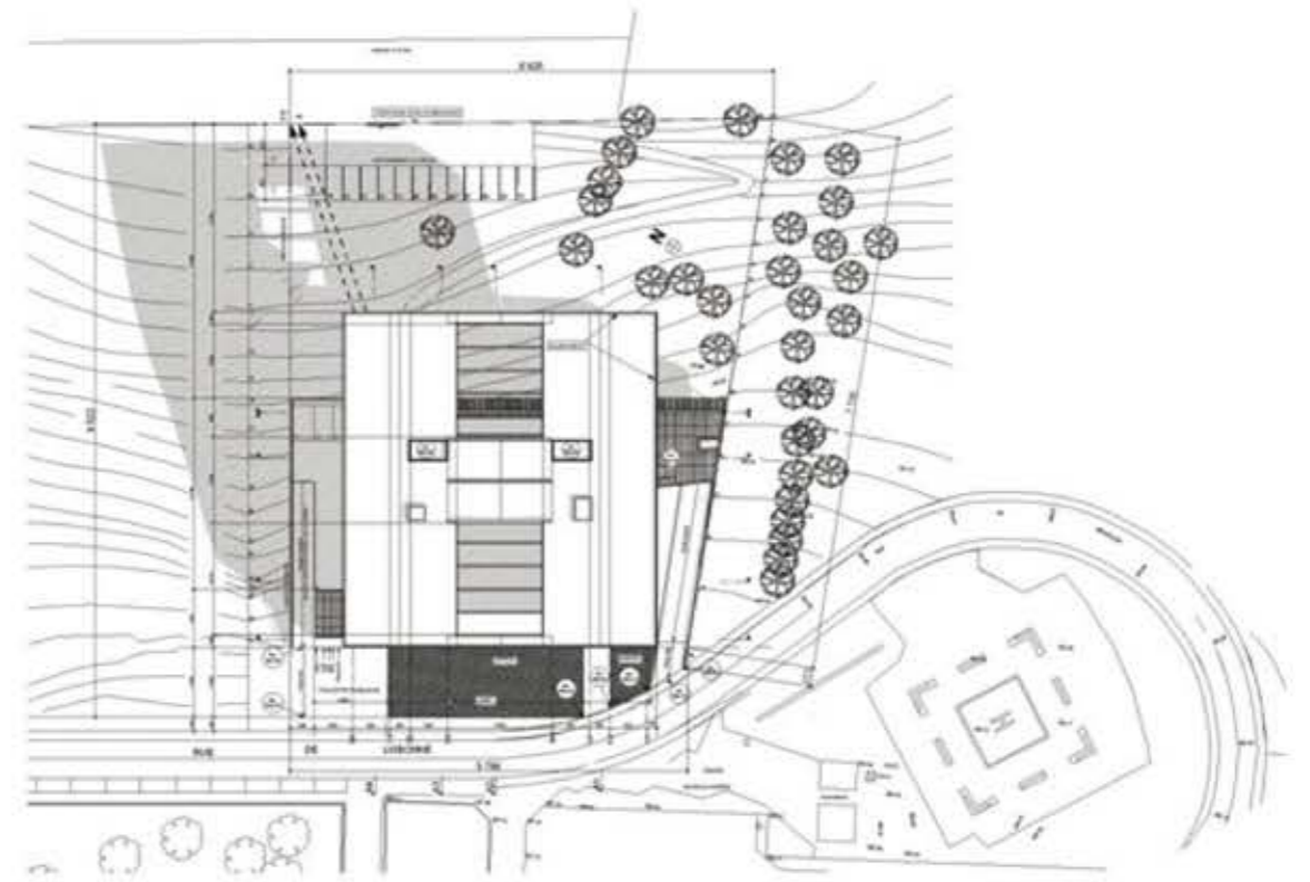
Mass plan
